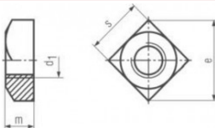
SQUARE NUT ( DIN-557 )
