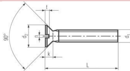
SOLTTED MACHINE SCREW ( DIN-963 )
