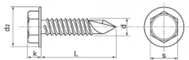
SELF DRILLING SCREW ( DIN-7504 )
