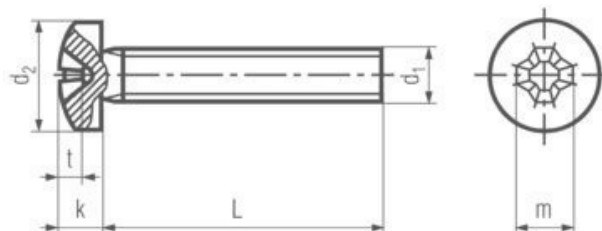
PHILLIPS PAN HEAD SCREW ( DIN-7985 )
