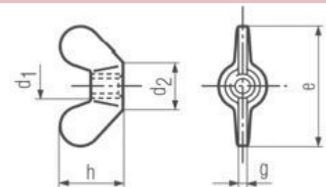
WING NUT ( DIN-315 )
