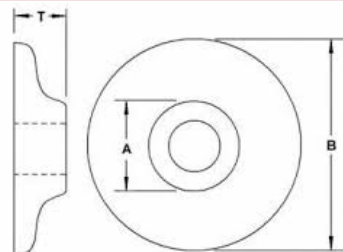
OGEE WASHER
