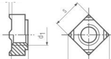
SQUARE WELD NUT ( DIN-928 )
