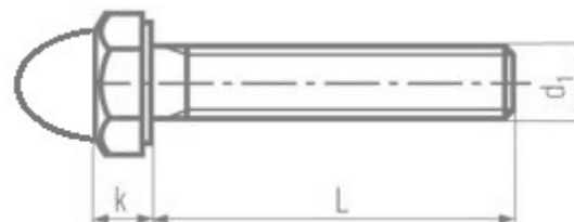
HEX DOME BOLT
