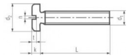
SLOTTED PAN HEAD SCREW ( DIN-85 )
